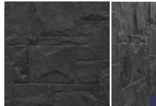
BLACK LIMESTONE
